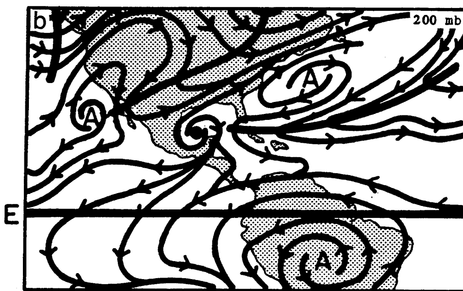
Fig. 6.5 Dual-channel outflow. (a) Idealized sketch of a dual outflow channel with the cyclone center to the west of the anticyclone center. (b) 200 mb streamlines for future hurricane Henri on 16 September 1979 which had a dual-channel outflow at the time. (Chen and Gray, 1985)
