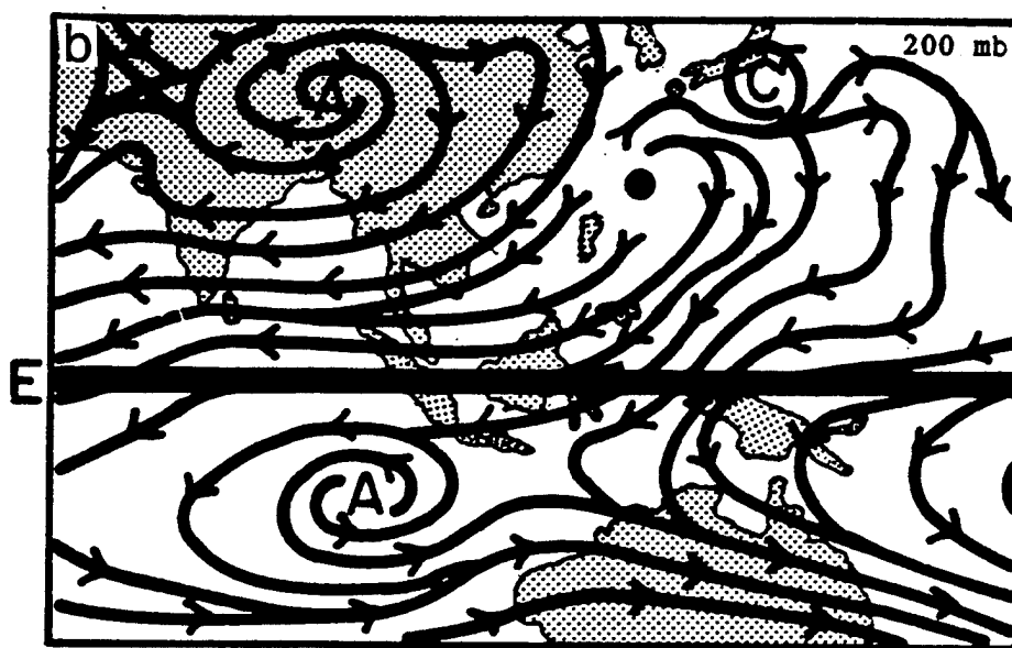
Fig. 6.4 Single-channel equatorward outflow. (a) Idealized sketch of a single equatorward outflow channel for a cyclone center to the east of the anticyclone center. (b) 200 mb streamlines for Typhoon Irving on 13 August 1979 that had single-channel equatorward outflow at the time. (Chen and Gray, 1985)
